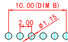
RECOMMENDED PCB LAYOUT TOP VIEW (. XX ± 0.05)
